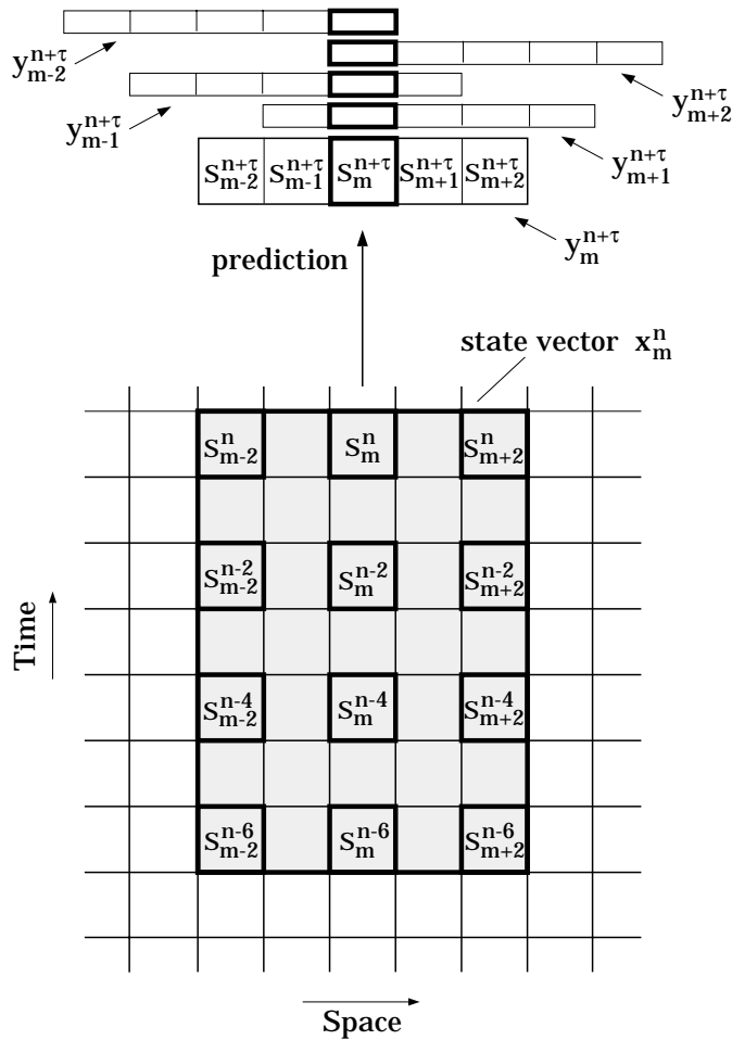
Figure 1: Local reconstruction of states from regions of the spatio-temporal time series S = \{\mathbf{s}^n\}^{n=1, \dots, N} = \{s_m^n\}_{m=1, \dots, M}^{n=1, \dots, N} and prediction of the future value of the center element s_m^{n+\tau} using forecasts of overlapping regions \dots, \mathbf{y}_{m-2}^{n+\tau}, \mathbf{y}_{m-1}^{n+\tau}, \mathbf{y}_m^{n+\tau}, \mathbf{y}_{m+1}^{n+\tau}, \mathbf{y}_{m+2}^{n+\tau}, \dots that give the future evolution of the center region and of neighboring regions.
